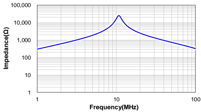
SPRH1210F-820M
