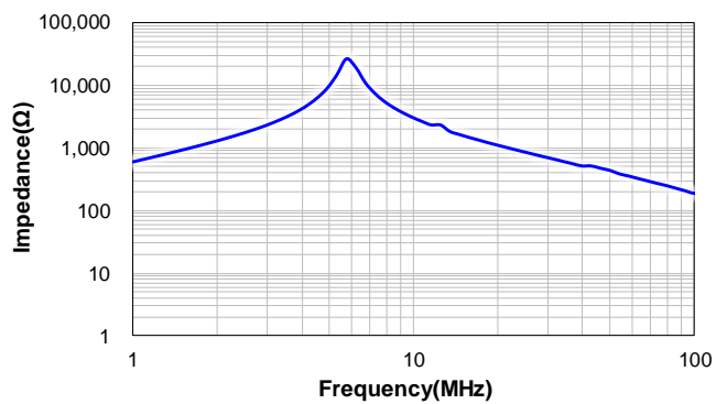
SPRH1210F-101M
