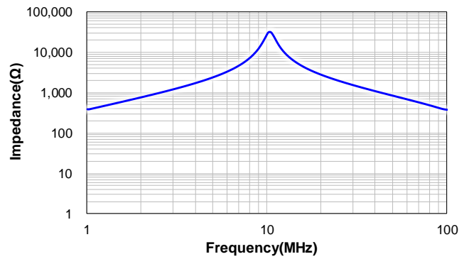
SPRH1210F-101M
