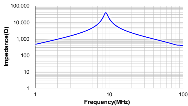
SPRH1210F-820M
