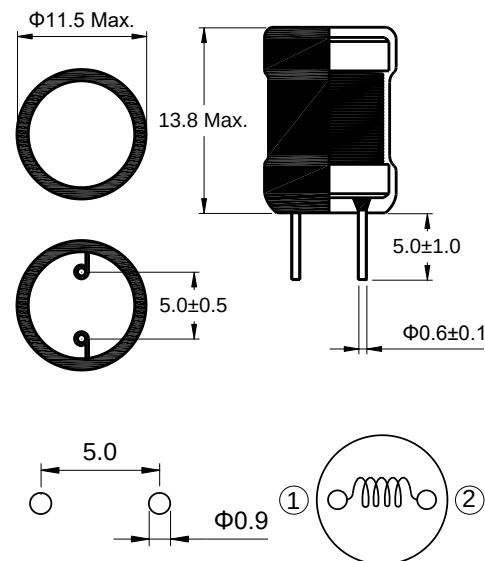
Typical Hole Pattern
