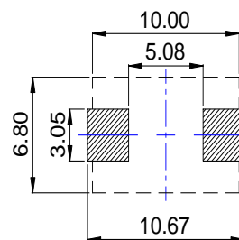
Reference Land Pattern
