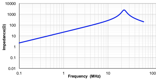
CSEB0530H-3R3M
