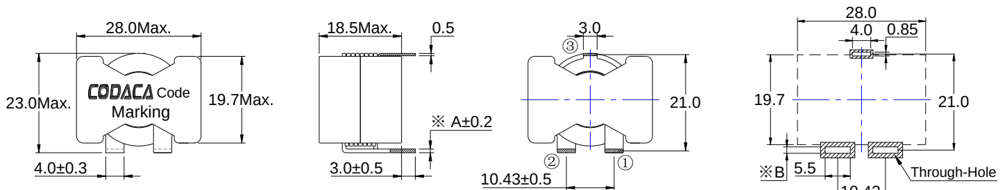
Reference Hole Pattern
