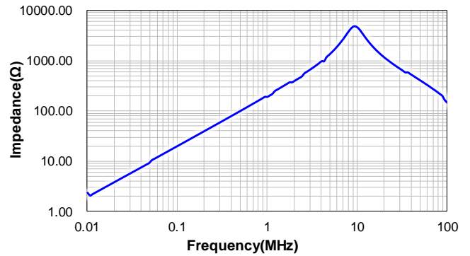
CPCF2920AS-680M
