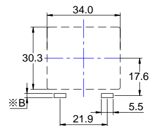
Reference Hole Pattern
