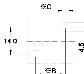
Typical Hole pattern
