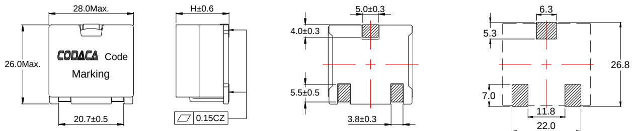
Reference Land Pattern
