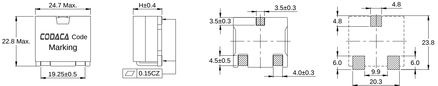
Reference Land Pattern
