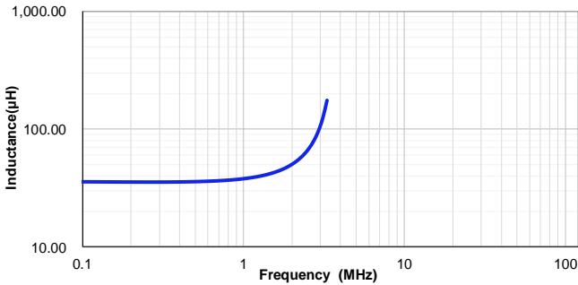
VSHB1054T-330MC
