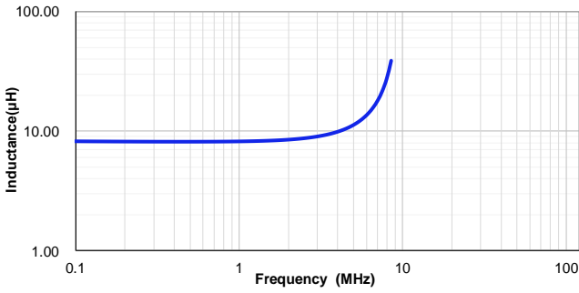
VSHB1054T-8R2MC
