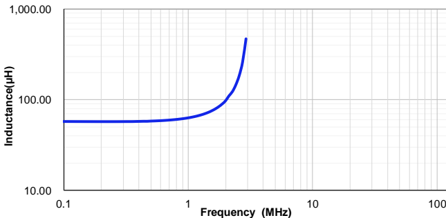
VSHB1054T-560MC
