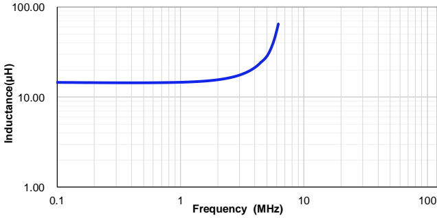
VSHB1054T-150MC
