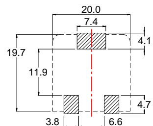
Reference Land Pattern
