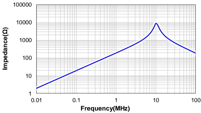
VSBX1275-320M
