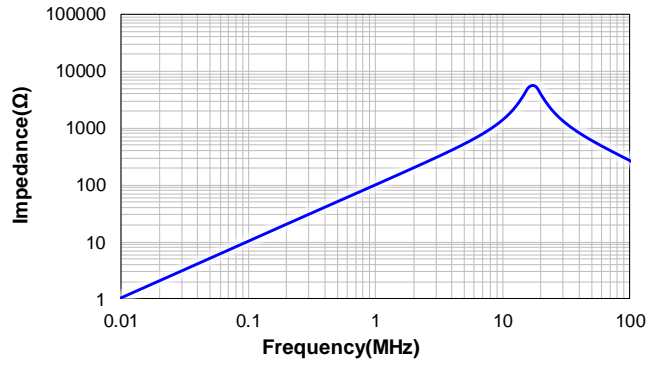
VSBX1275-250M
