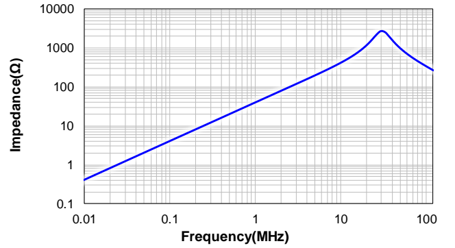
VSBX1275-100M
