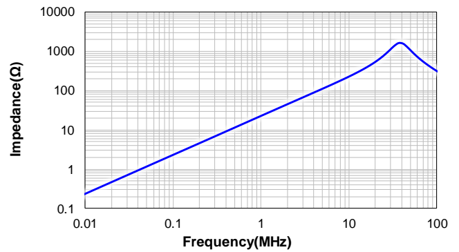
VSBX1275-6R8M
