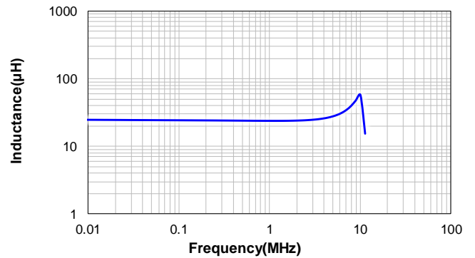
VSBX1275-250M
