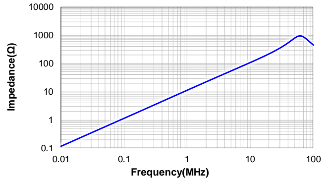
VSBX1275-3R9M
