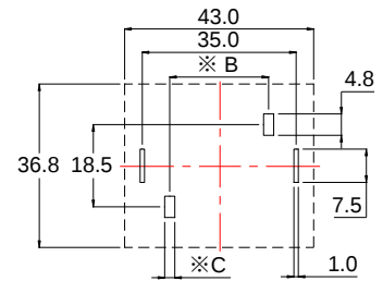
Reference Hole Pattern
