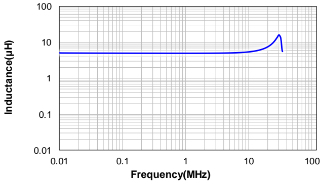
VPRX2520SP-5R6MC
