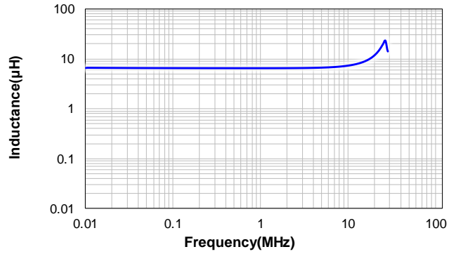
VPRX2520SP-6R8MC
