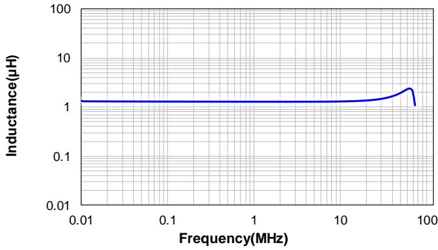
VPRX2520SP-3R0MC
