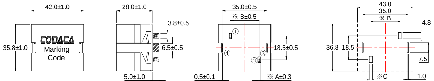
Reference Land Pattern
