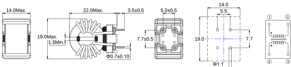
Reference Hole Pattern
