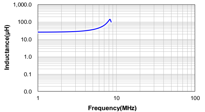
CSUC1210-270M:270M
