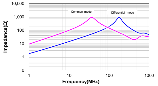
CSUC1210-3R6M:3R6M
