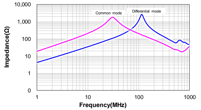
CSUC1210-6R0M:6R0M
