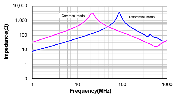
CSUC1210-6R0M:6R0M
