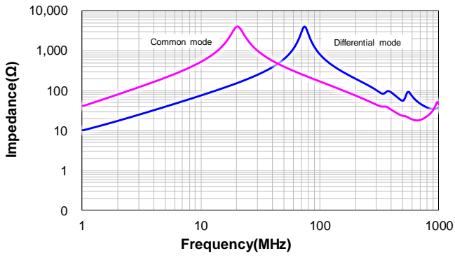
CSUC1210-130M:130M
