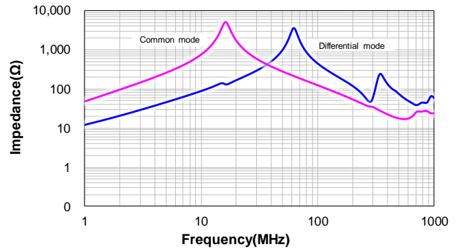
CSUC1210-150M:150M
