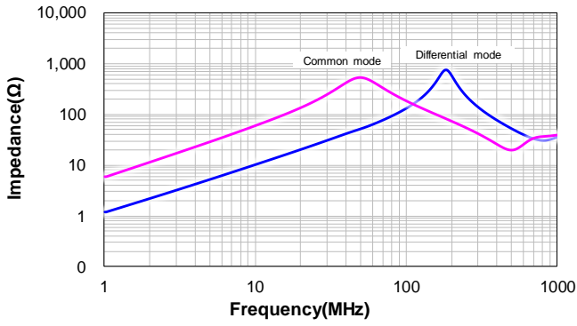
CSUC1210-2R4M:2R4M
