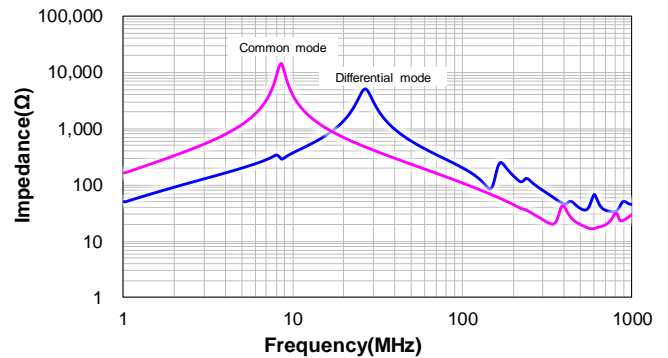
CSUC1210-270M:270M
