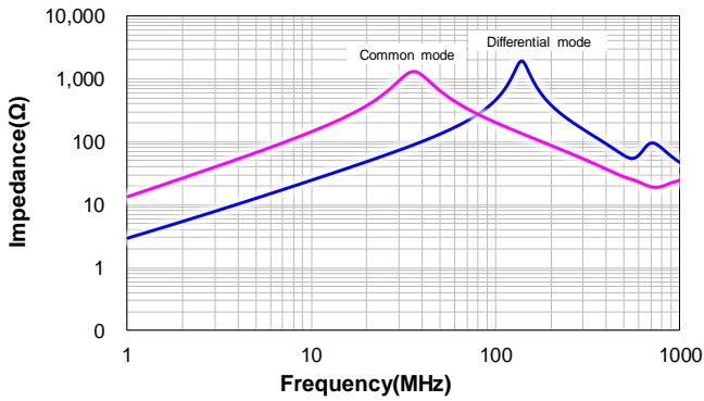
CSUC1210-4R7M:4R7M
