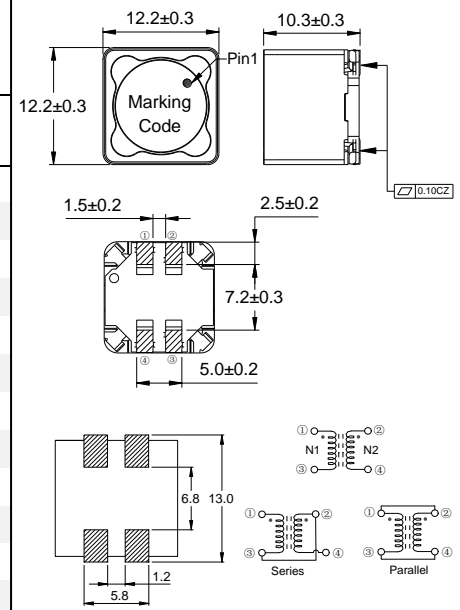
Typical Land Pattern
