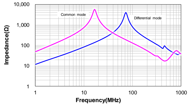
CSUC1208-8R6M:8R6M
