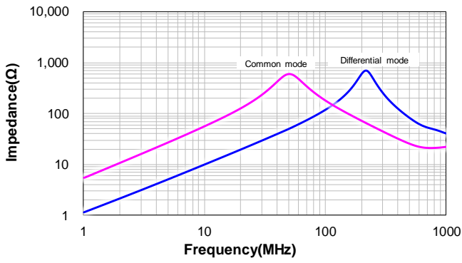
CSUC1208-2R4M:2R4M
