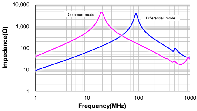
CSUC1208-120M:120M
