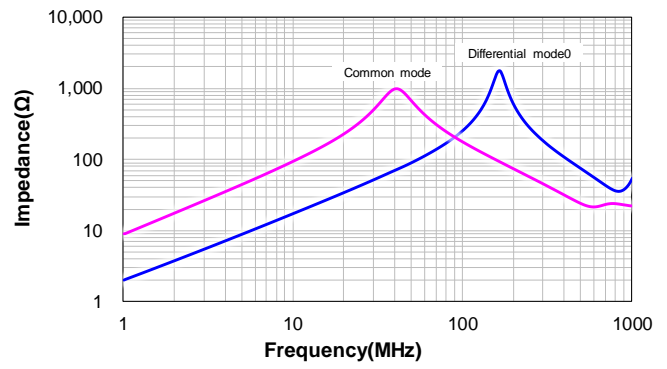
CSUC1208-3R3M:3R3M
