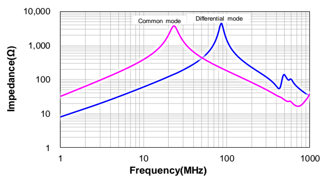
CSUC1208-5R6M:5R6M
