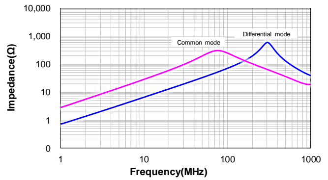
CSUC1208-1R6M:1R6M
