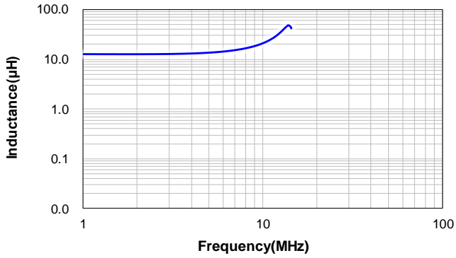
CSUC1208-120M:120M
