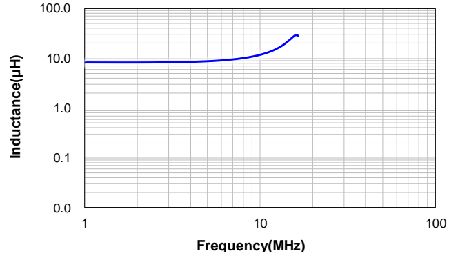
CSUC1208-8R6M:8R6M
