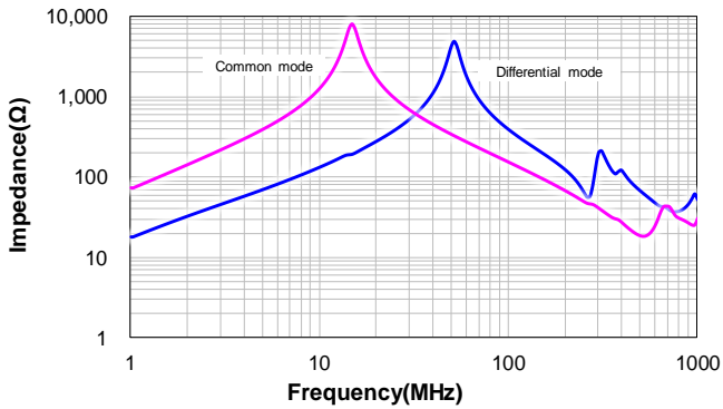
CSUC1208-120M:120M
