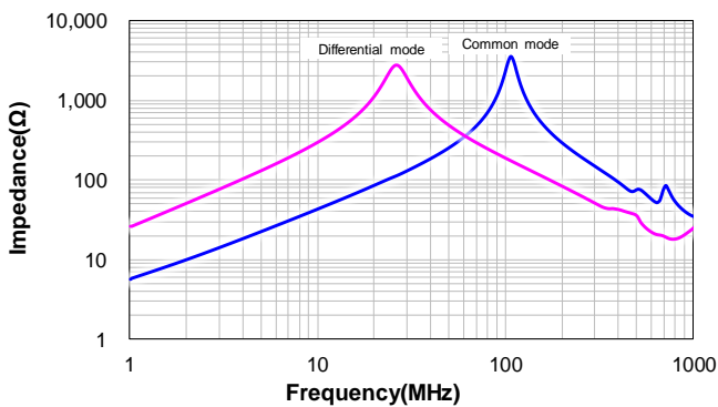
CSUC1208-4R7M:4R7M
