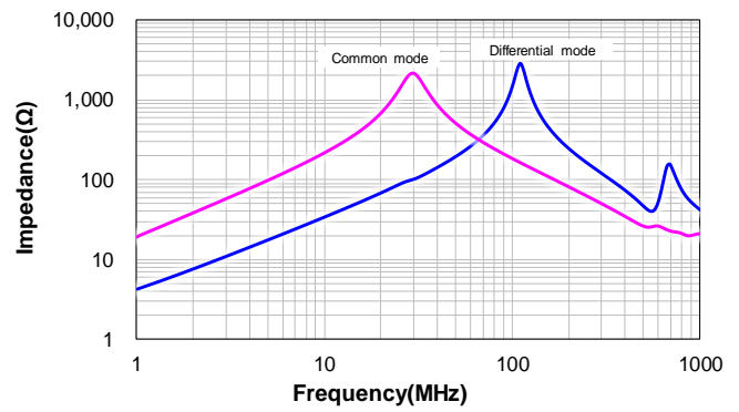
CSUC1208-5R6M:5R6M
