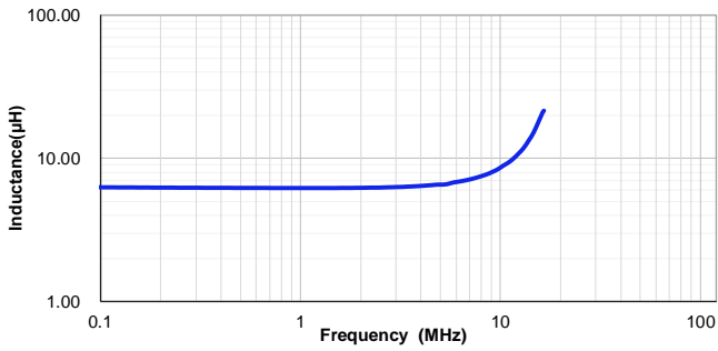
CSEB0730-6R8M
