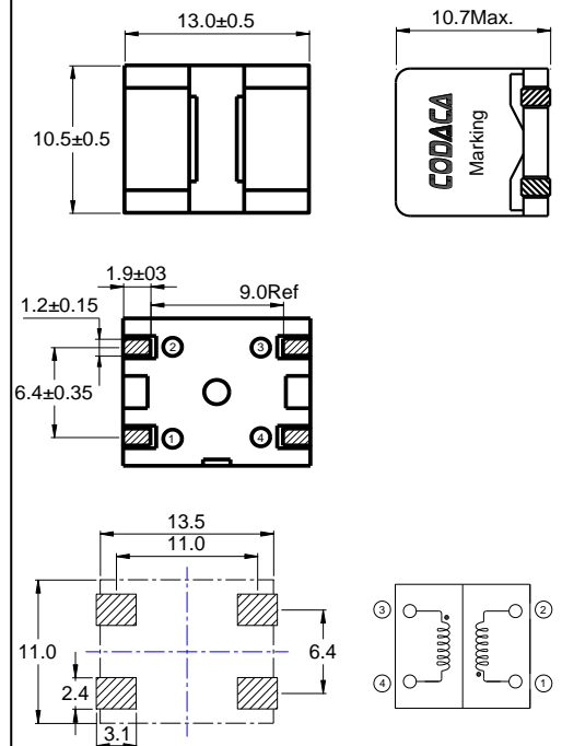
Reference Land Pattern
