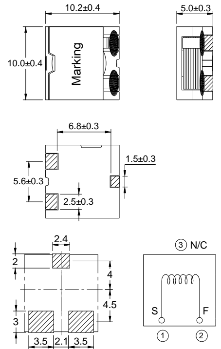
Typical Land Pattern
