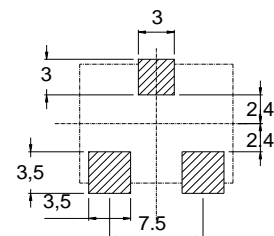
Typical Land Pattern
