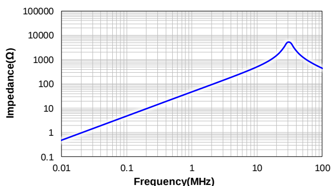
CSBA0860-8R0M
