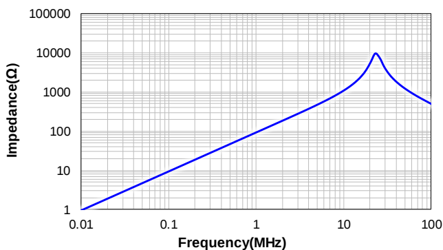
CSBA0860-150M
