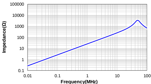
CSBA0860-4R3M
