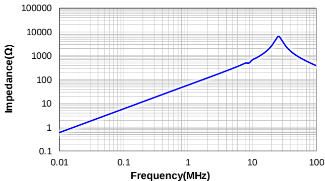
CSBA0860-100M
