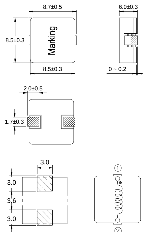
Typical Land Pattern
