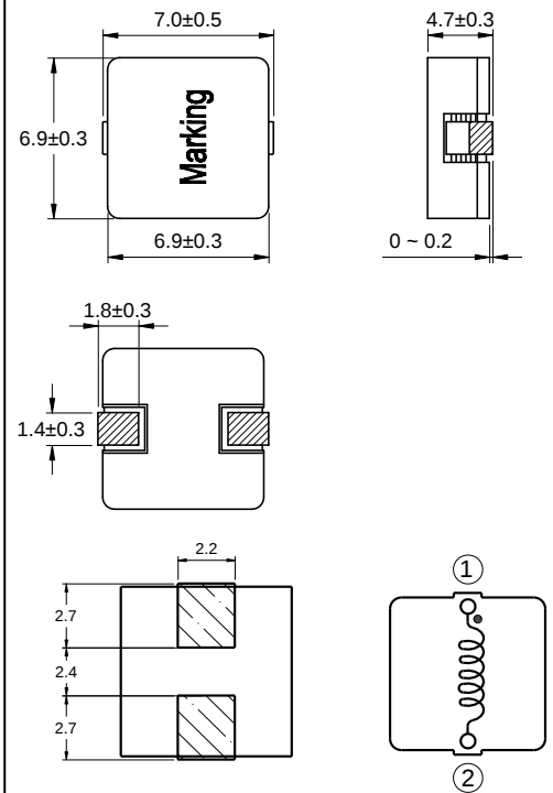
Typical Land Pattern
