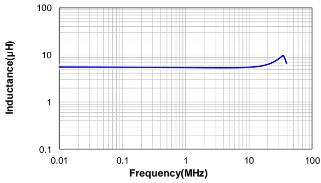
CSBA0640-5R5M
