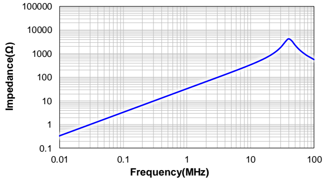
CSBA0640-5R5M
