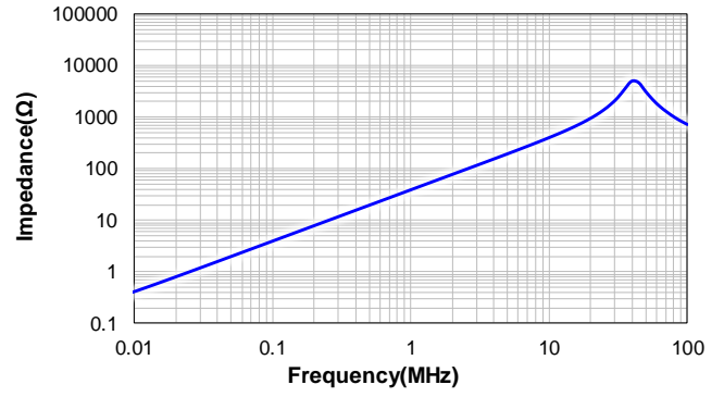
CSBA0640-6R5M
