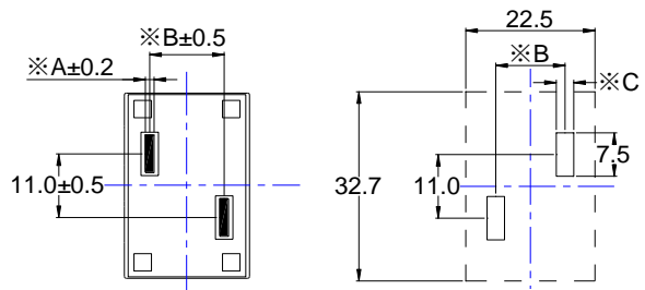
Reference Hole Pattern
